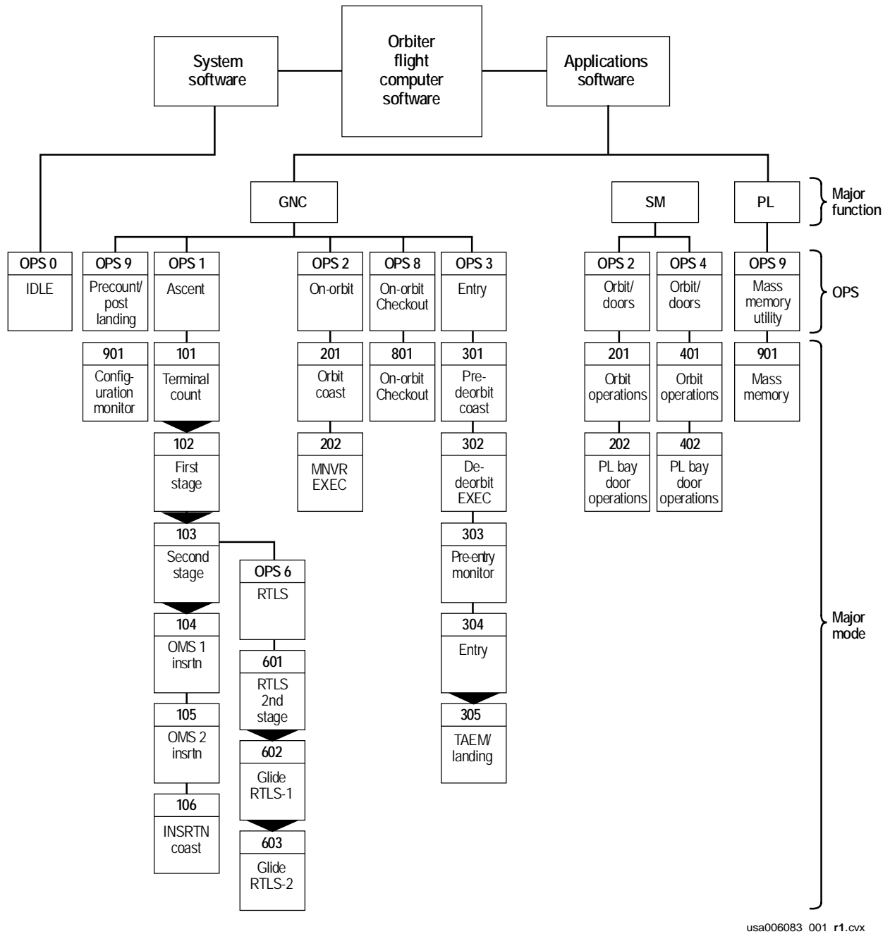
Figure 1-1. PASS software structure
