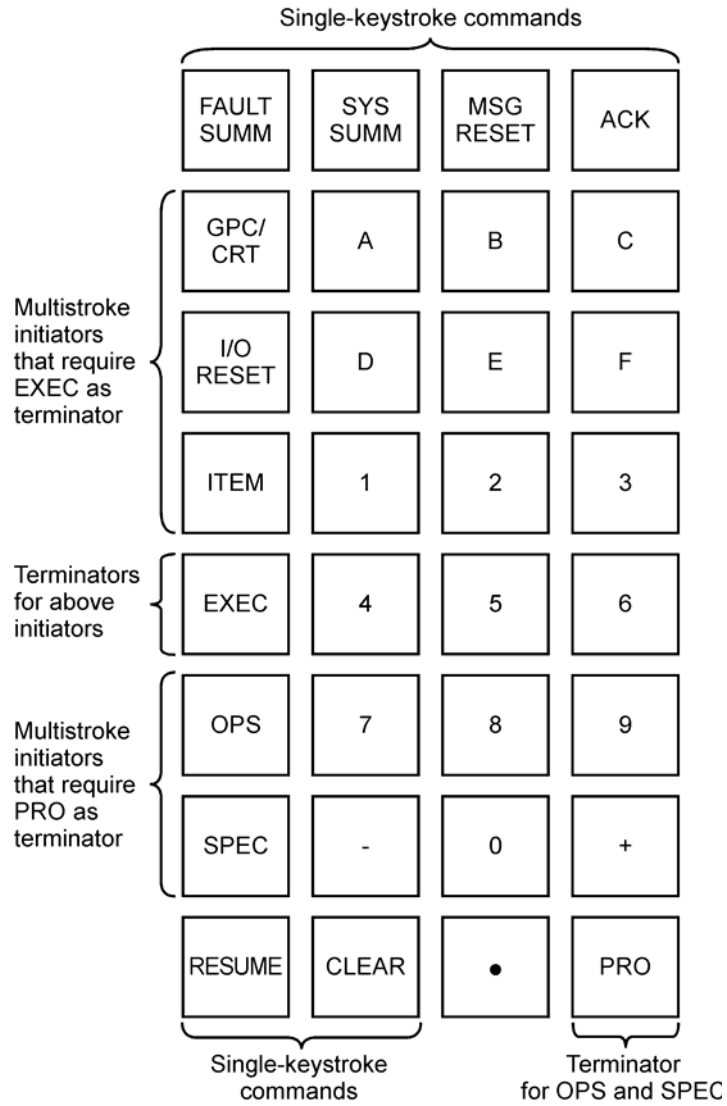
Figure 2-4. Keyboard found on panels C2 and R11
