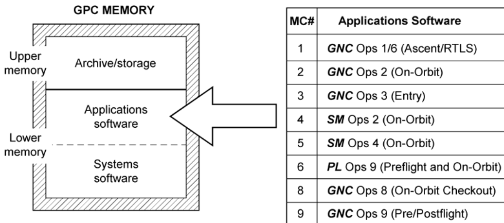
Figure 1-3. GPC memory and applications software memory configurations
