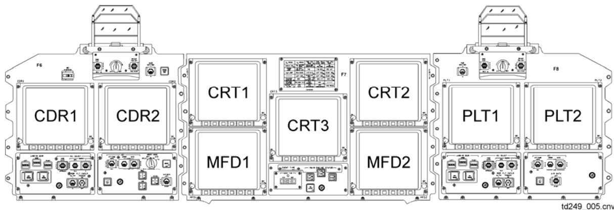
Figure 2-1. Forward cockpit displays
